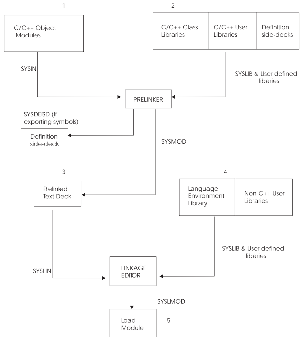
Figure 49. Basic prelinker and linkage editor processing
