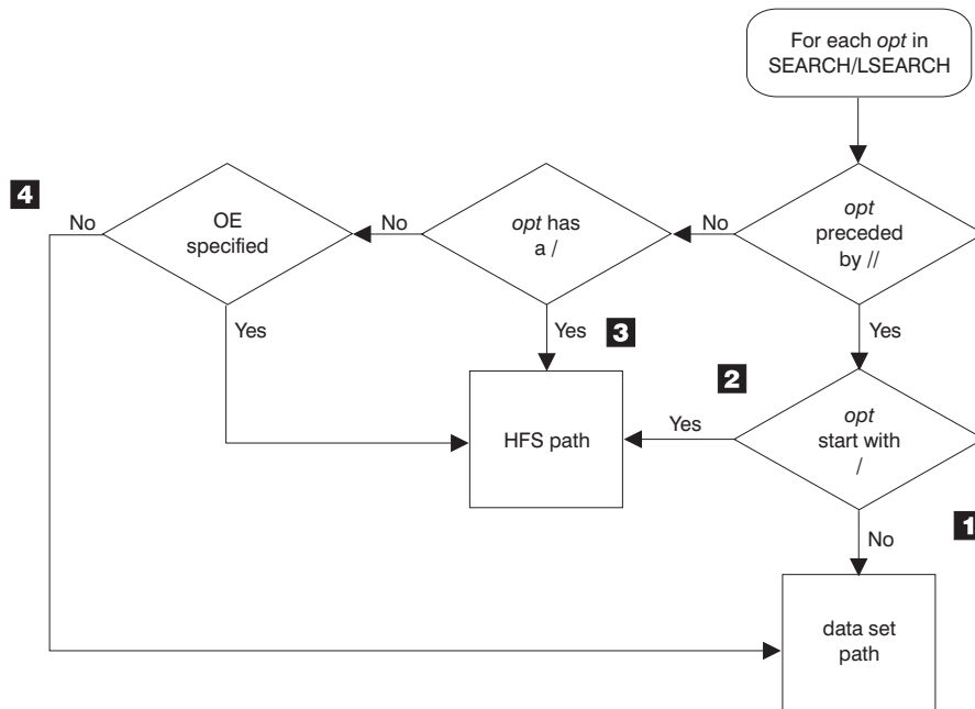
Figure 25. Determining if the SEARCH/LSEARCH opt is a z/OS UNIX path
